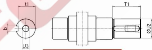
单输出轴/Single output shaft
